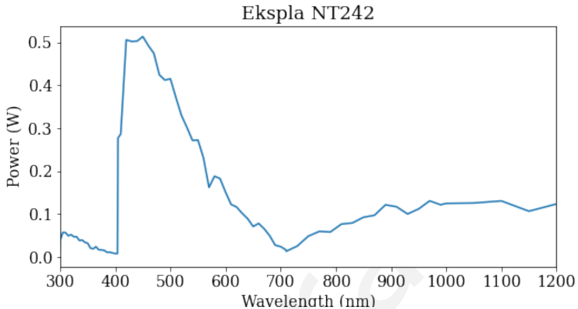
Figure 1: Expected Power output of NT242 Tunable Laser
